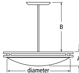
SO suspension
