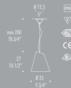
MICENE S25 AL max 1x100W- 250V E27
