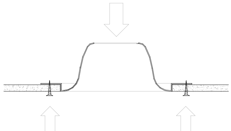
SECTION
