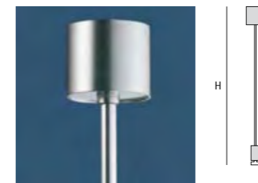
SILVER Ø H* SX 99-820-3 10mm 600 SX 99-821-3 10mm 1200 SX 99-822-3 13mm 600 SX 99-823-3 13mm 1200
