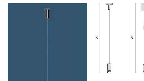
SILVER S* SX 99-830-3 Wire suspension 1500 SX 99-831-3 3000 SX 99-824-3 with 3 core supply cable (3 x 0.75²) 1500 SX 99-825-3 3000 SX 99-826-3 with 5 core supply cable (5 x 1.5²) 1500 SX 99-827-3 3000
