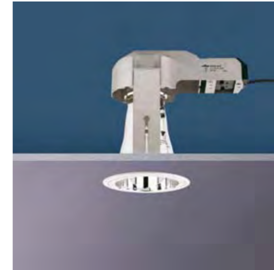
DOWNLIGHT WITH VERTICAL LAMP POSITION
