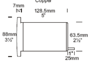
Copper Fluorescent Option
