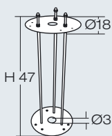
code 0404M003 Loop in loop out IP68
