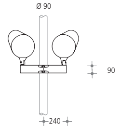
OLIVIO Grande SX 810 Double lateral projector
