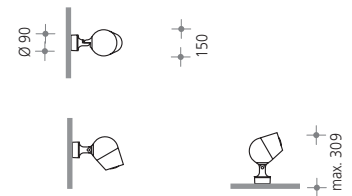
OLIVIO Piccolo SX 792 / SX 809 Surface mounted fitting
