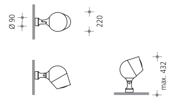
OLIVIO Medio SX 791 / SX 808 Surface mounted fitting
